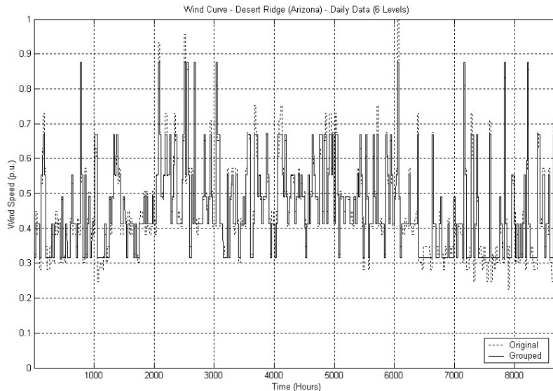
Figure 2: Wind Curve – Desert Ridge (Arizona) – Daily Data – Original Curve and Grouped into 6 Levels
