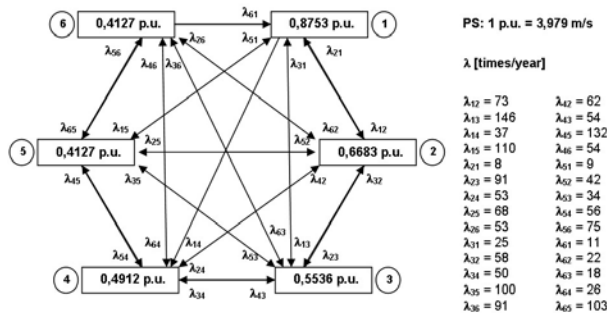
Figure 3: States Transition Diagram of the Wind Generation
