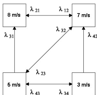
Figure 1: Wind States Transition Diagram
