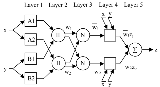
Figure 3: ANFIS architecture.
