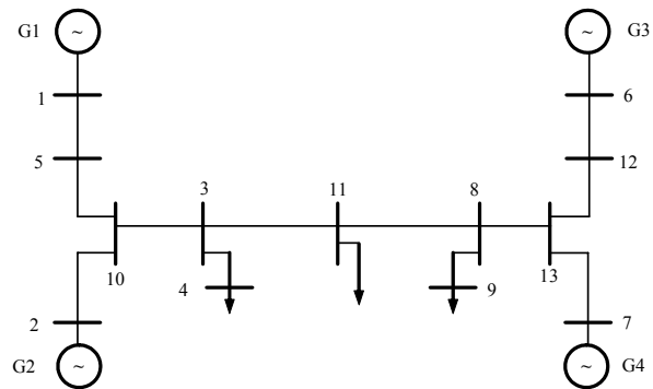
Figure 2: Four-machine two-area power system model
