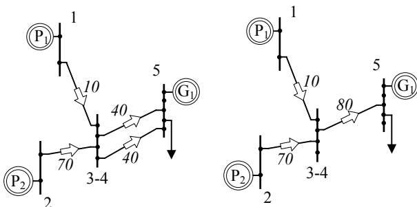
Figure 11: N and N-1 results for the preventive mode ( \alpha = 1 ).
