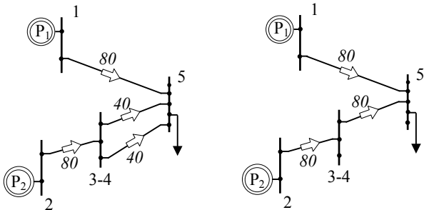
Figure 10: N and N-1 results for the preventive mode ( \alpha = 0 ).
