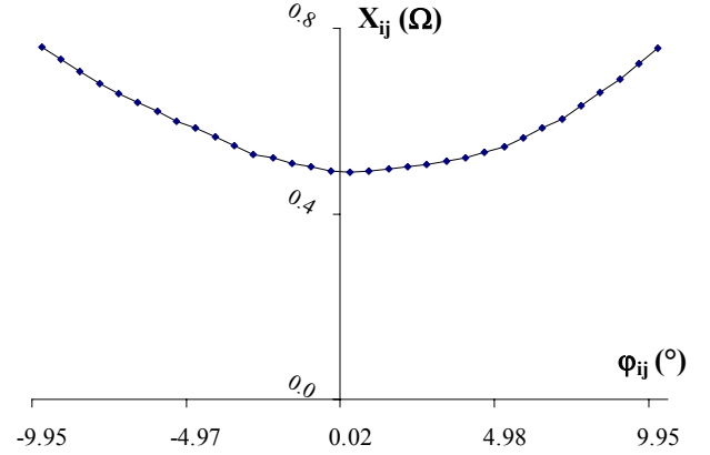
Figure 17: Phase shifting transformer reactance as a function of the phase for 33 taps.
