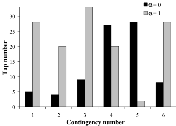
Figure 18: Tap results for each contingency.
