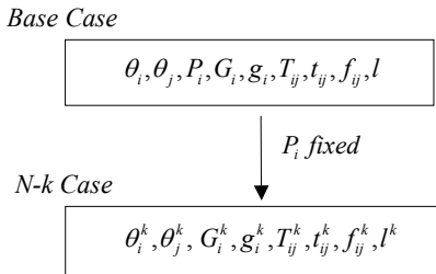
Figure 7: Variables treatment in curative mode.
