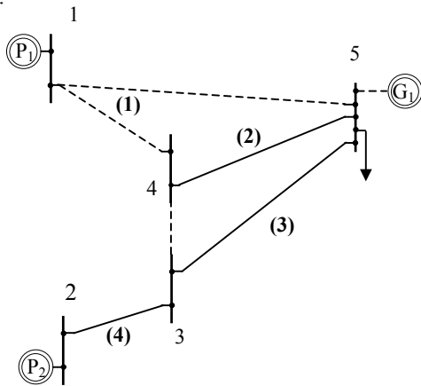
Figure 8: 5-buses test system.
