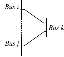
Figure 4: The buses i and j are split: f_{ij} = 0 .
