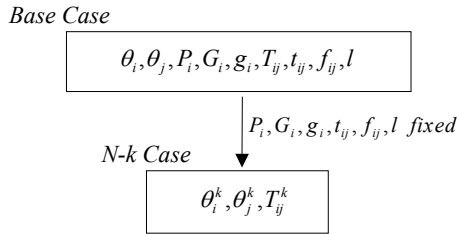
Figure 6: Variables treatment in preventive mode.
