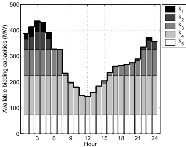
Figure 1: Available bidding capacities after preplanning
