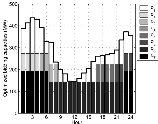
Figure 2: Optimized spot and reserve market bidding capacities
