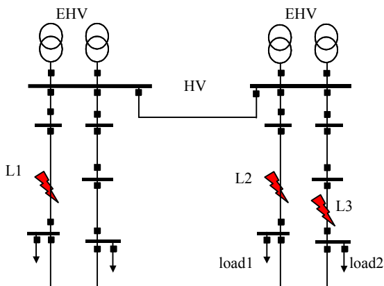
Figure 3: Consequences of outage combinations in comparison to those of single outages
