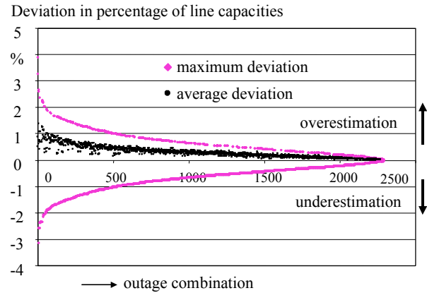
Figure 6: Deviation of the load flow estimation
