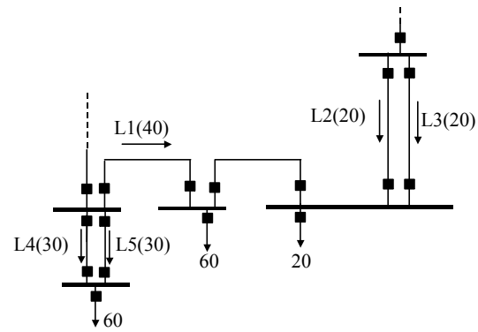
Figure 5: Estimation of load flow after outage combinations
