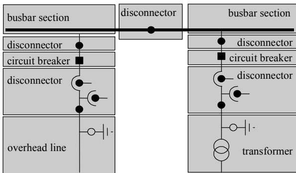
Figure 1: Modeling of electrical networks in reliability analysis
