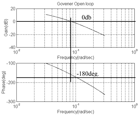
Figure 14: Governor system frequency characteristic of pumped storage hydraulic generator under application to PID constants in Table 6 with permanent droop
