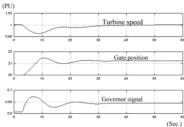
Figure 13: Governor response to 5% step-wise load increase from generator 80% load with improved PID
