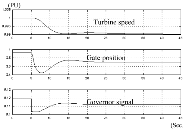
Figure 8: Governor response simulation at -1% step change
