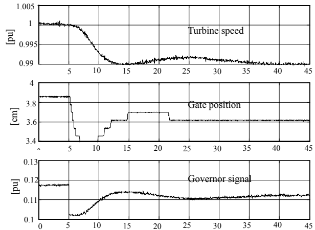
Figure 7: Governor response test record at -1% step change (Sec.)
