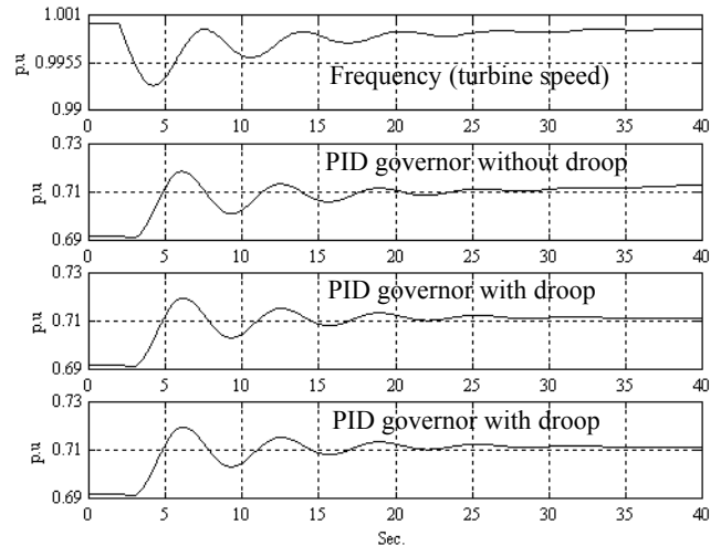
Figure 17: Governor response to 5% step-wise load increase from generator 60% load (100% is a total generator capacity of three generators.)
