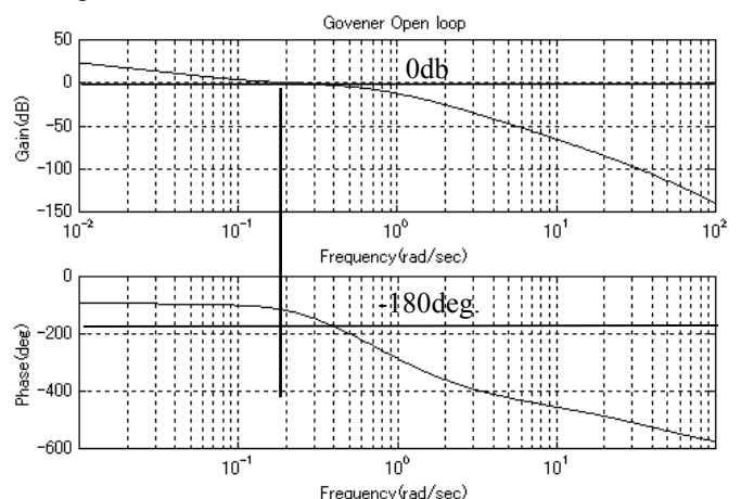
Figure 11: Governor system frequency characteristic of pumped storage hydraulic generator under application to new designed PID constants
