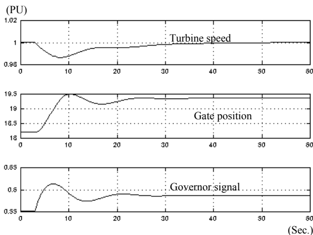
Figure 12: Governor response to 5% step-wise load increase from generator 60% load with improved PID
