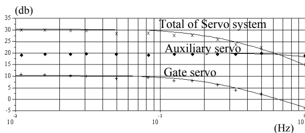
Figure 5: Servo system frequency characteristic of 250MW pumped storage hydraulic generator-measured
