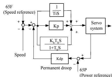
Figure 2: PID governor
