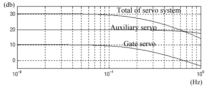
Figure 6: Servo system frequency characteristic of the 250MW pumped storage hydraulic generator calculated based on the measured data
