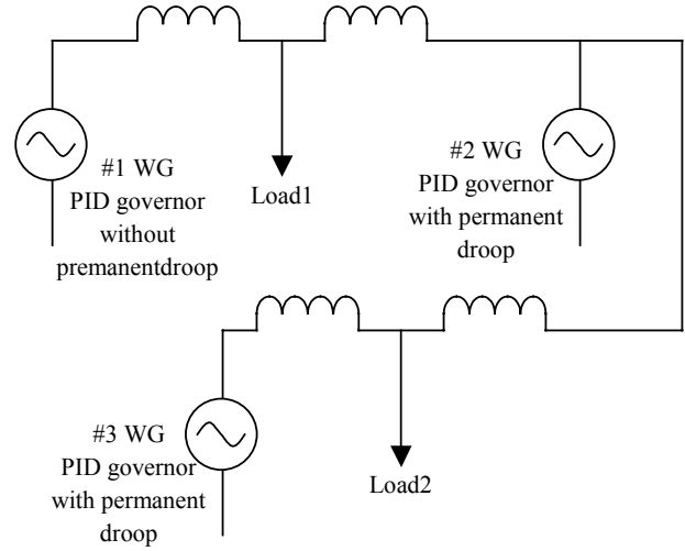
Figure 16: Three machines power system configuration with PID governor
