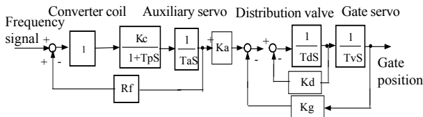
Figure 4: Frequency response test configuration using the actual servo system (under stopping of the turbine generator)
