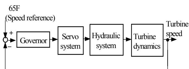
Figure 1: Governor system configuration with turbine dynamics
