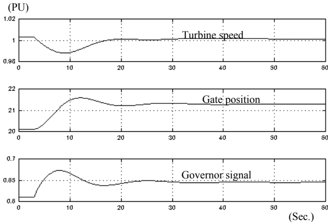
Figure 15: Governor response to 5% step-wise load increase from generator 80% load with PID in Table 6 with permanent droop
