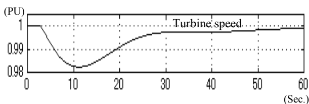
Figure 9: Governor response to 5% step-wise load increase from generator 60% load
