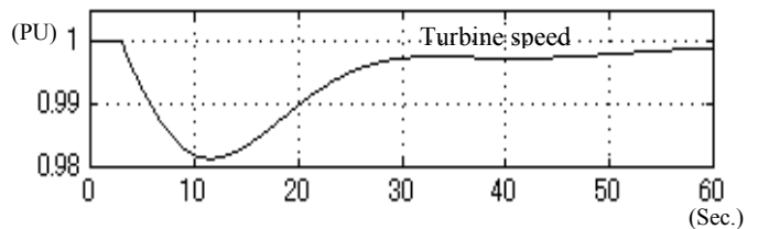
Figure 10: Governor response to 5% step-wise load increase from generator 80% load
