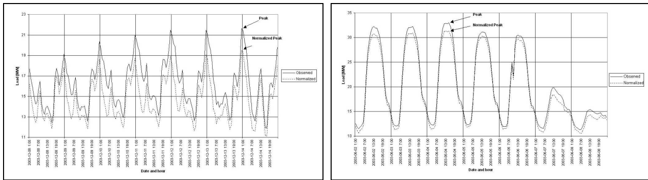
Figure 2: Load patterns (Observed and Adjusted) during the week of the yearly peak for LOAD1 (Left) and LOAD2 (Right).
