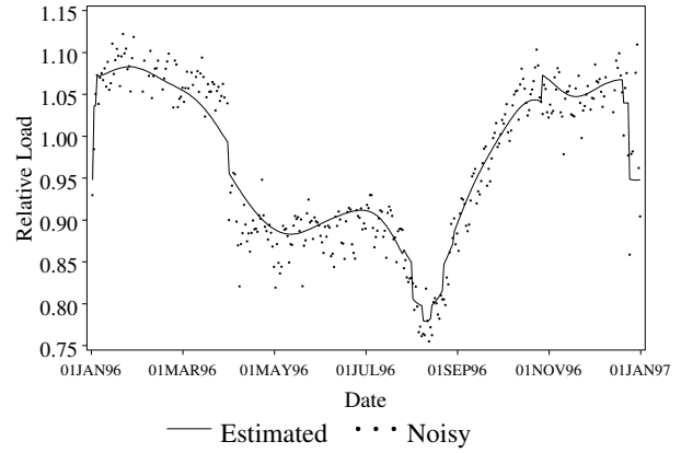
Figure 2: Seasonality at 19h, in 1996 : noisy \tilde{S} and estimated S .
