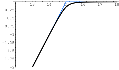
Figure 1: Threshold function \underline{\psi} with t = 15 and \sigma = 0.5 .
