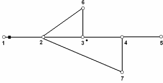
Figure 1: Network diagram for the 7-bus system
