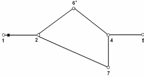
Figure 2: System diagram after the merger of buses 3 and 6.
