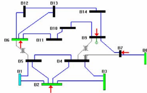
Figure 3: PMU locations for the 14 bus system (ignoring zero injections).
