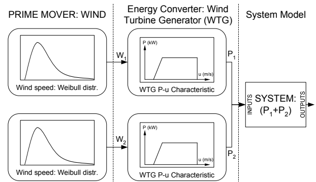
Figure 3: Stochastic Generation Modelling Procedure (Case of WTGs)
