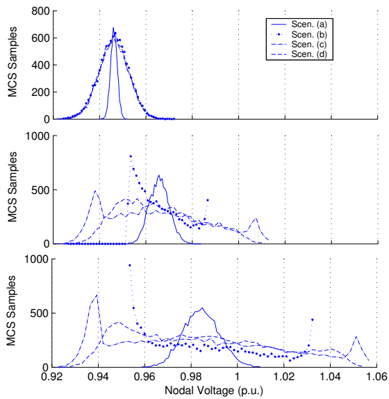
Figure 9: Voltage Distributions for Node 40, for three penetration levels of wind power
