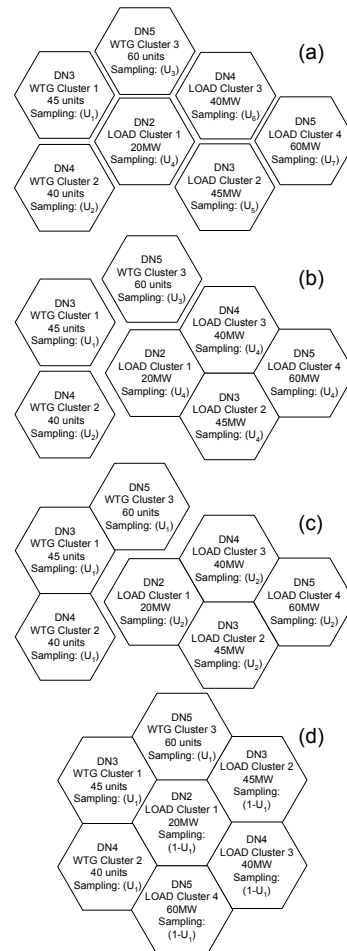
Figure 13: Clusters for system upper bound stochastic modelling
