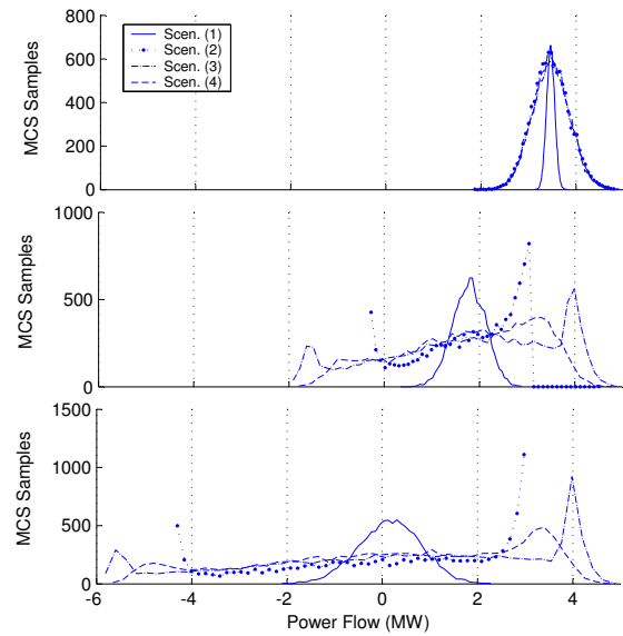
Figure 11: Power Flow Distributions for Branch 47-43, for three penetration levels of wind power
