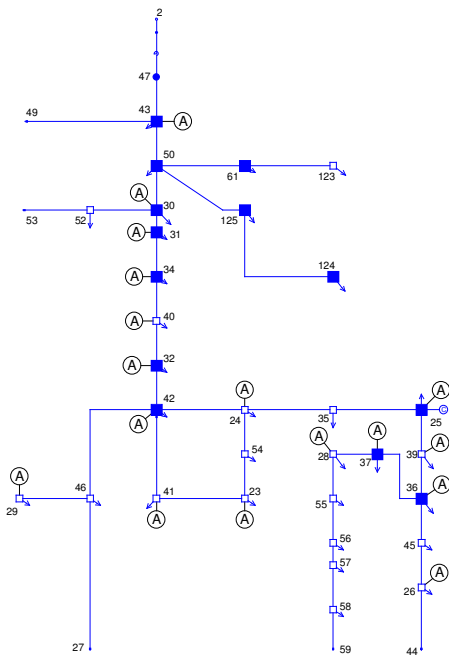
Figure 8: Study Case 1: 34-bus 38-branch Distribution System
