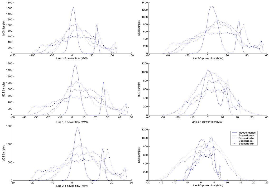
Figure 14: Power Flow Distributions for the system lines
