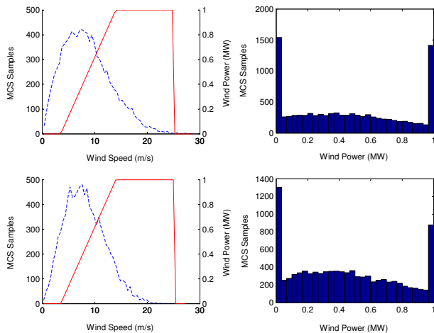
Figure 4: Wind Speed Distributions, WTG Wind Speed - Power Characteristic, WTG Power Output Distributions for the WTGs
