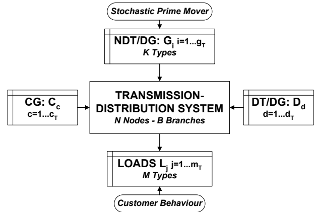
Figure 2: Power System Schematic Representation
