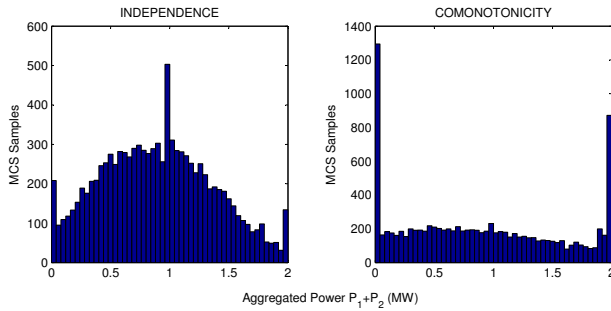
Figure 6: Aggregated Power Output from two Stochastic Generators
