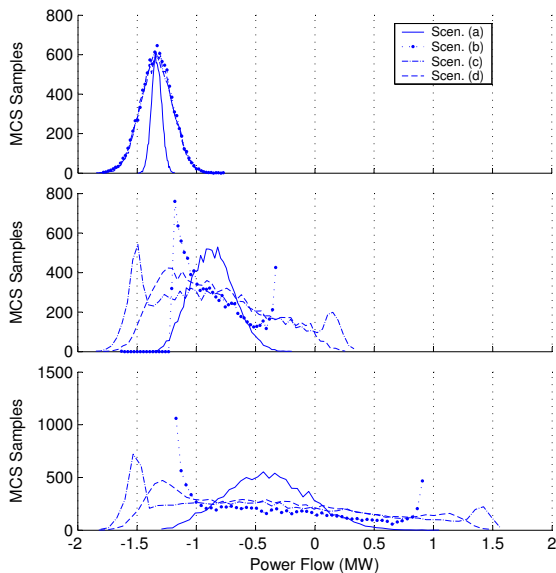
Figure 10: Power Flow Distributions for Branch 39-25, for three penetration levels of wind power
