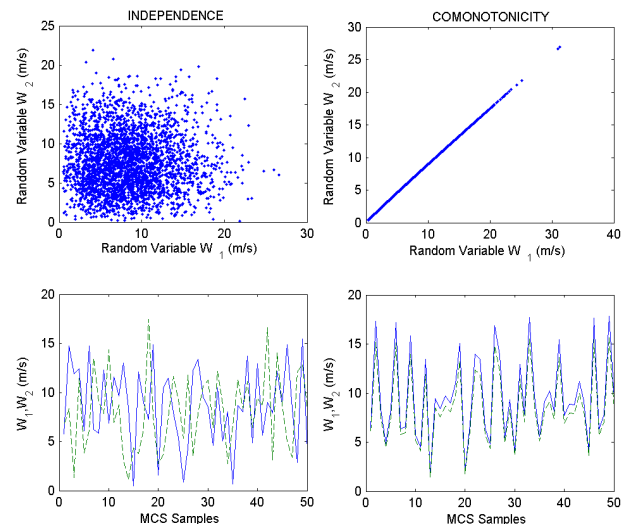
Figure 5: Scatter-plots and time-series data for the two dependence scenarios
