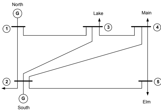
Figure 12: 5-bus / 7-branch Test System (Hale Network)
