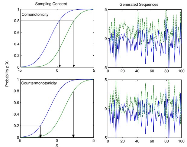
Figure 7: Comonotonic/Countermonotonic Sampling and Generated Sequences
