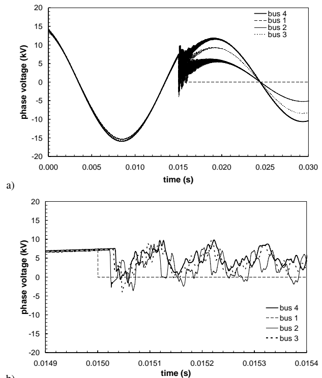
Figure 2 Voltage transients on a phase due to a three-phase fault at bus 1 as observed at three different nodes (bus 2, bus 3 and bus 4), of the power distribution network shown in Figure 1: a) general behavior, b) detailed view.
