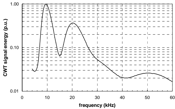
Figure 3 Results of the CWT analysis of the voltage transient of Figure 2 at bus 4. The values are in per unit with respect to the maximum ( 1.25 \cdot 10^{12} V 2 s).
