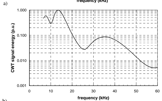
Figure 6 Results of the CWT analysis of mode 0 of the voltage transient at bus 4, due to a phase-to ground fault at bus 1: a) grounded neutral network, b) ungrounded neutral. The values are in per unit with respect to the maximum ( 1.37 \cdot 10^9 V 2 s and 1.74 \cdot 10^{11} V 2 s for the case of grounded and ungrounded neutral, respectively).
