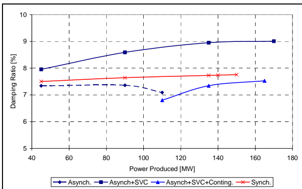
Figure 2: Damping ratio vs. power produced at the G1 terminals. 100 MVA rated machine, area 1 importing from area 2
