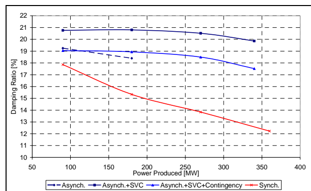
Figure 13: Damping ratio vs. power produced at the G1's terminals. 200 MVA rated machine export case T=5.4 sec.
