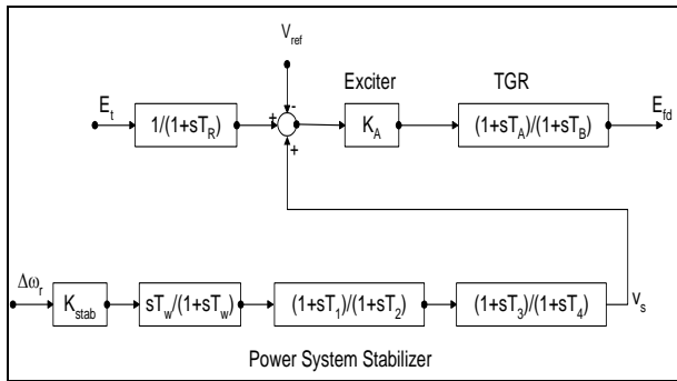
Figure 17 Power System Stabilizer (PSS) block diagram. K_{STAB}=20 ; T_w=10 ; T_1=0.05 ; T_2=0.02 ; T_3=3 ; T_4=5.4 ;
