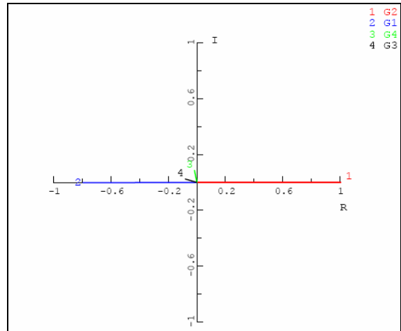
Figure 14 Local mode of oscillation in area 1 corresponding to the eigenvalue -2.63326, +j0.978334 Hz.
