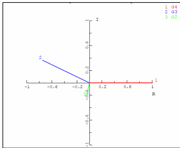
Figure 15: Local mode of oscillation in area 2 corresponding to the eigenvalue 1.41062, +j1.19376 Hz.
