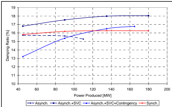
Figure 10: Damping ratio vs. power produced at the G1's terminals. 100 MVA rated machine. Import case T=5.4 sec.
