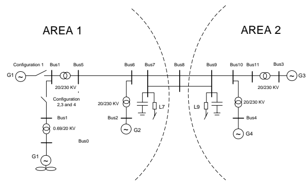
Figure 1 Four generator test system
