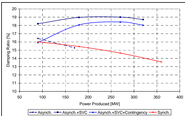
Figure 11: Damping ratio vs. power produced at the G1's terminals. 200 MVA rated machine. Import case T = 5.4 sec.
