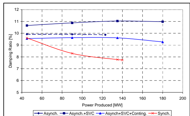
Figure 6: Damping ratio vs. power produced at the G1's terminals. 100 MVA rated machine, area 1 exporting to area 2.
