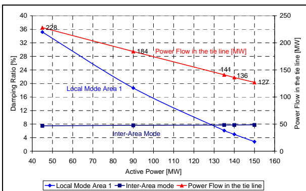
Figure 4: Configuration 1- Oscillation modes and power flow in the tie line between bus7 and bus8 as a function of the active power produced at G1's. 100 MVA rated synchronous machine, area 1 importing from area 2.
