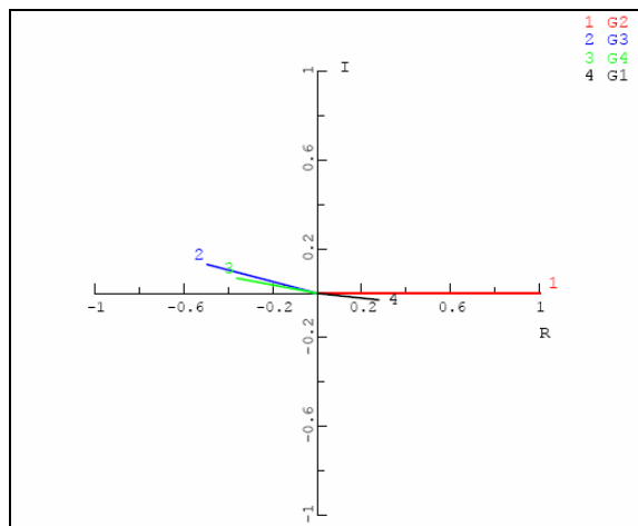
Figure 16: Inter-area mode of oscillation between area 1 and area 2 corresponding to the eigenvalue -0.608954, +j0.597950 Hz.
