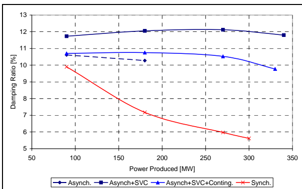
Figure 7: Damping ratio vs. power produced at the G1's terminals. 200 MVA rated machine, area 1 exporting to area 2
