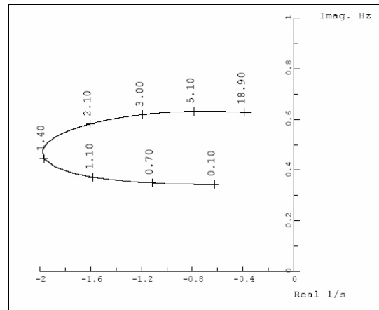
Figure 8: Root loci of the eigenvalue corresponding to the inter-area mode as affected by the PSS time constant T4. Curve parameterised with T4.
