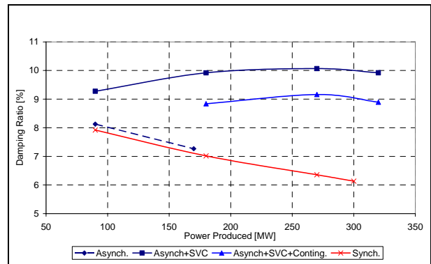
Figure 5: Damping ratio vs. power produced at the G1's terminals. 200 MVA rated machine, area 1 importing from area 2.
