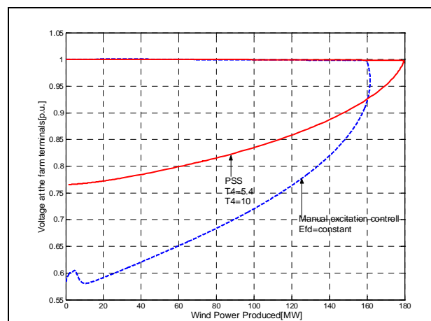
Figure 9: P-V curves with automatic voltage regulator and PSS (as affected by PSS tuning) and without voltage regulator (manual excitation control)
