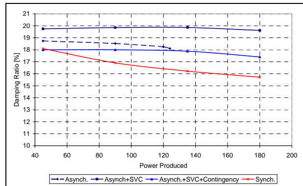
Figure 12: Damping ratio vs. power produced at the G1's terminals. 100 MVA rated machine export case T=5.4 sec.
