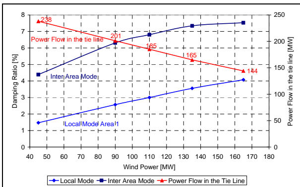
Figure 3: Configuration 4- Oscillation modes and power flow in the tie line between bus7 and bus8 as a function of the active power produced at the G1's terminals. 100 MVA rated asynchronous machine, contingency case with area 1 importing from area 2.
