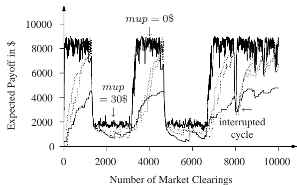
Figure 8: Evolution of the Q -function for G_2 (3 active agents)
