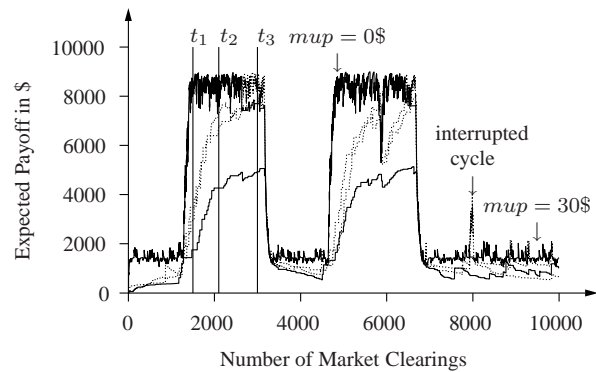
Figure 7: Evolution of the Q -function for G_1 (3 active agents)
