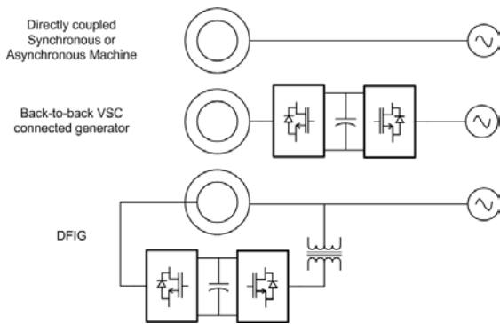
Figure 1: Wind generator technologies
