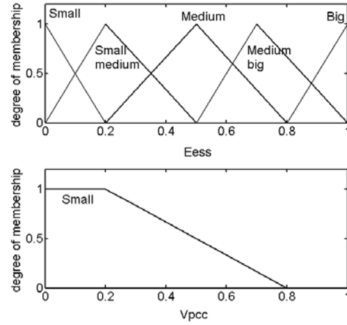
Figure 4: Membership functions for stored energy, E_{ess} , and the voltage at point of common coupling, V_{pcc} .
