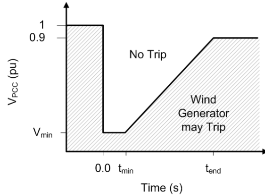
Figure 2: LVRT characteristic
