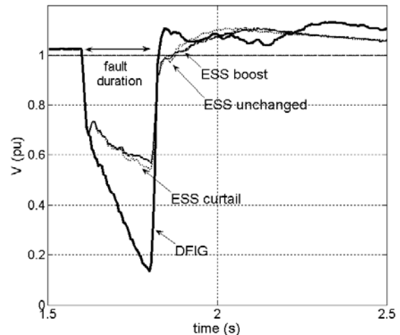
Figure 8: Response of voltage magnitude at PCC for (a) crowbar, (b) ESS – power boost, (c) ESS – curtailed power, and (d) ESS – P no change. SCR = 3, 12 cycle two-phase fault (1.6 to 1.8 s).
