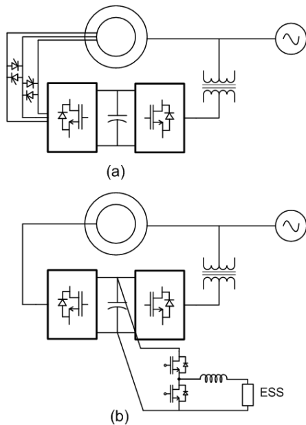
Figure 3: Possible realisations of LVRT characteristic in doubly-fed induction generator
