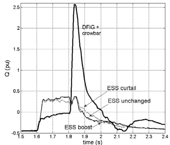
Figure 9: Reactive power delivered during two-phase, 12 cycle fault (1.6 to 1.8 s) for four cases.
