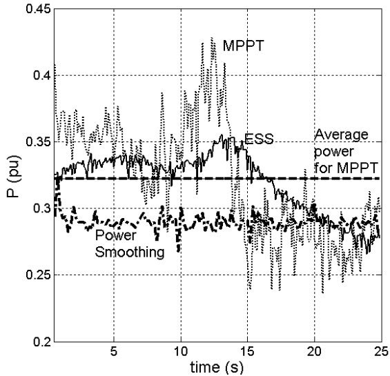
Figure 7: Grid power for (a) DFIG operating with MPPT algorithm, (b) DFIG with ESS operating using proposed algorithm and (c) DFIG operating with power smoothing algorithm.
