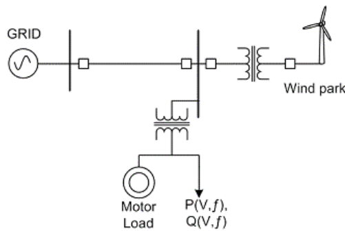
Figure 5: Interconnection of wind energy to medium voltage transmission network used for system studies.
