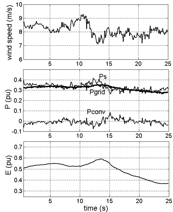
Figure 6: Normal operation showing (a) wind speed, (b) generator output power and (c) storage level for ESS.
