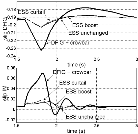
Figure 10: Response of generator (top) and motor load (bottom) slips during two phase, 12 cycle fault (1.6 to 1.8 s) for four cases.
