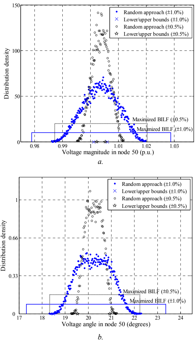
Figure 2: Probability densities in change of solutions (with respect to nominal, non-perturbed case) as a function of random perturbations in SCADA measurements and network branch parameters, compared with maximized BILF solution from Tables 1 and 2 and heuristic lower/upper bounds solution for uncertainty: 1) \pm 0.5\% and 2) \pm 1.0\% :
