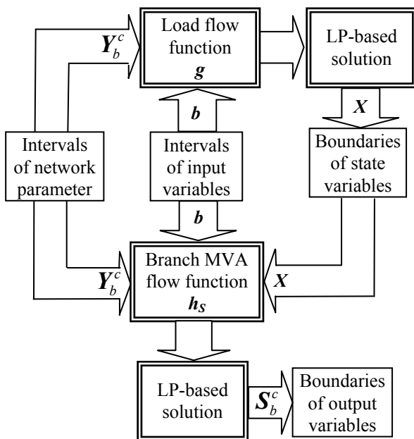
Figure 1: The flow-chart of BILF.
