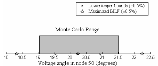
Figure 3: Monte Carlo versus LP predictions, bus 50, 0.5% perturbation.
