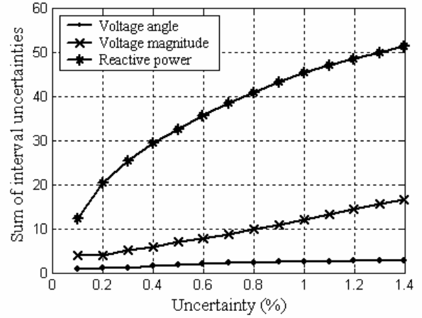
Figure 4: Sum of interval widths of various quantities as a function of the level of input uncertainty (Case 1 in Table 4).
