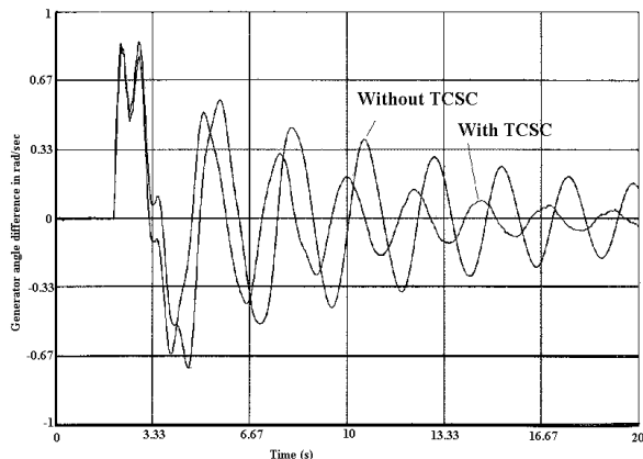
Figure 12: Damping on outage of HVDC line with the voltage based controller on RTDS.
