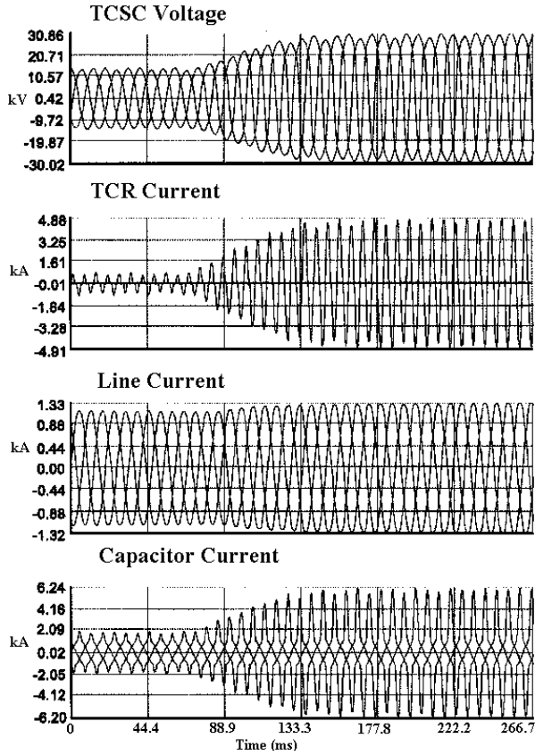
Figure 5: Step increase in the impedance setting.
