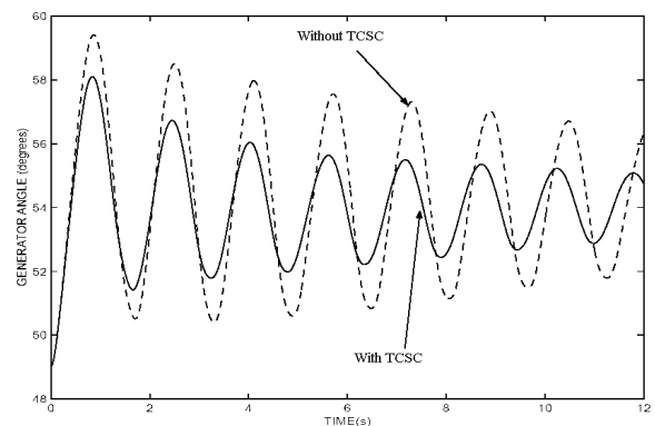
Figure 10: Damping on outage of HVDC line with the current based controller on MATLAB.
