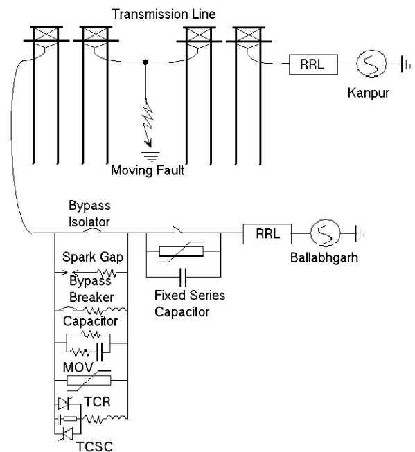
Figure 2: Simplified representation of the line, FSC and TCSC RTDS models.
