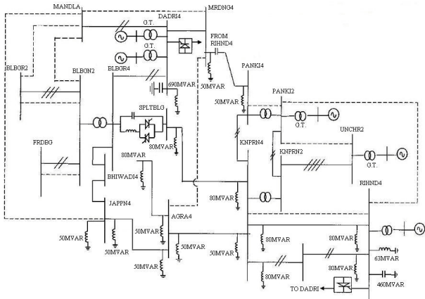
Figure 3: Reduced network representation
