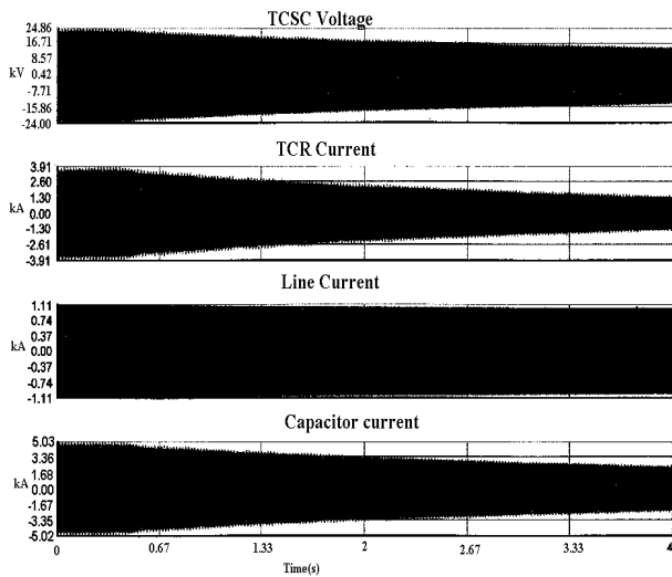
Figure 8: Step decrease in the current setting
