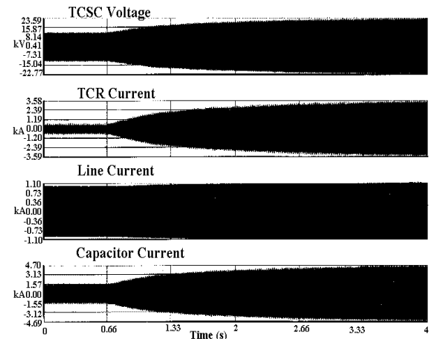
Figure 7: Step increase in the current setting.
