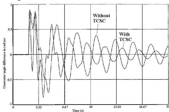
Figure 13: Damping on outage of HVDC line with the current based controller on RTDS.
