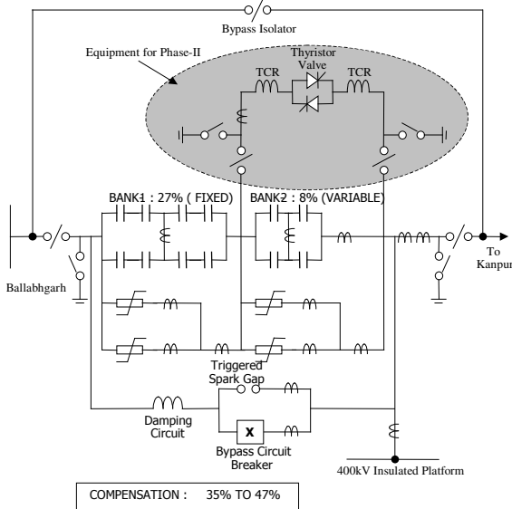
Figure 1: Single line diagram of the TCSC scheme.
