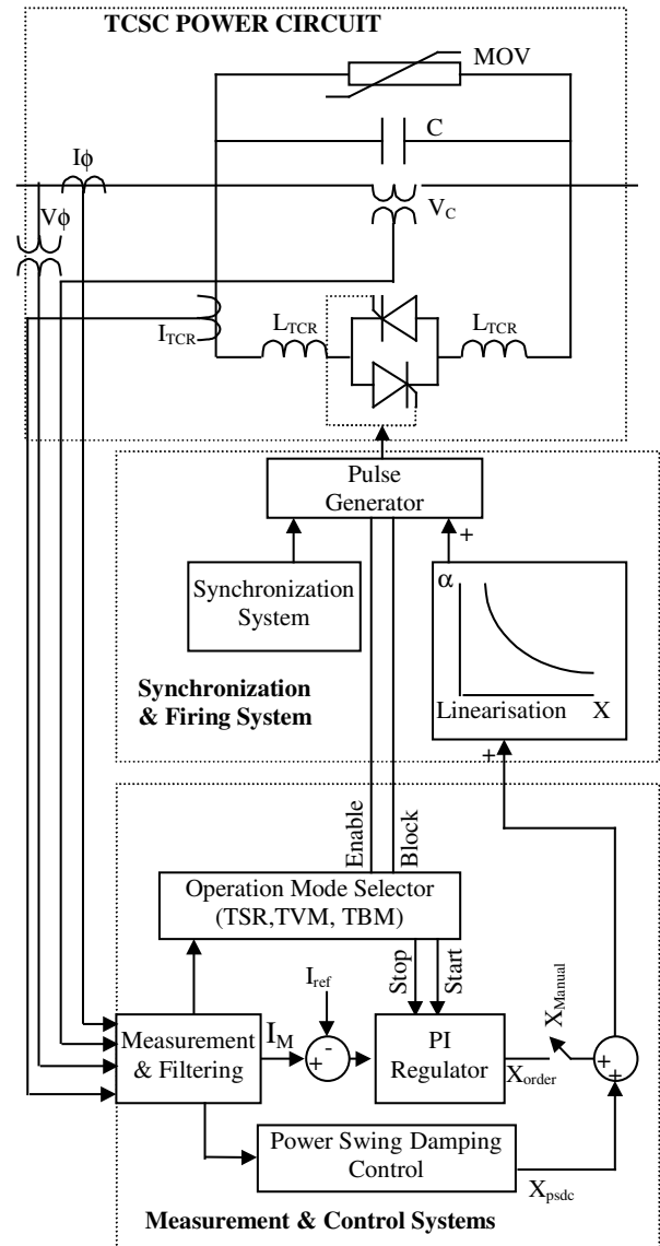
Figure 4: Block schematic of the TCSC and its control system.
