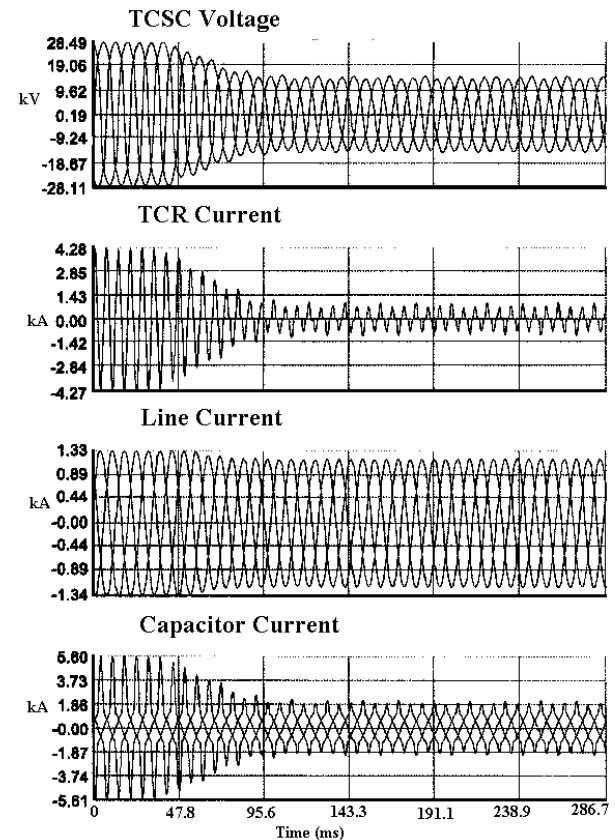
Figure 6: Step decrease in the impedance setting.
