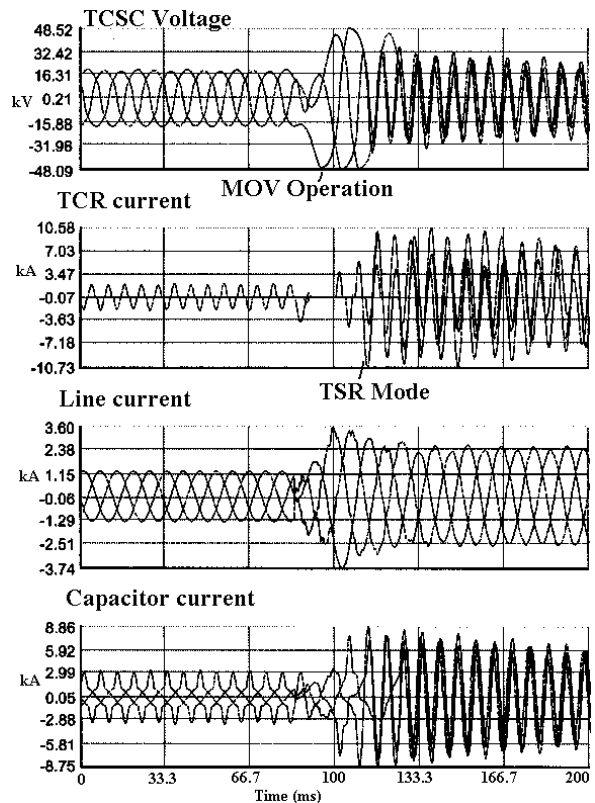
Figure 9: Three phase to ground fault on the Kanpur – Ballabgarh transmission line.
