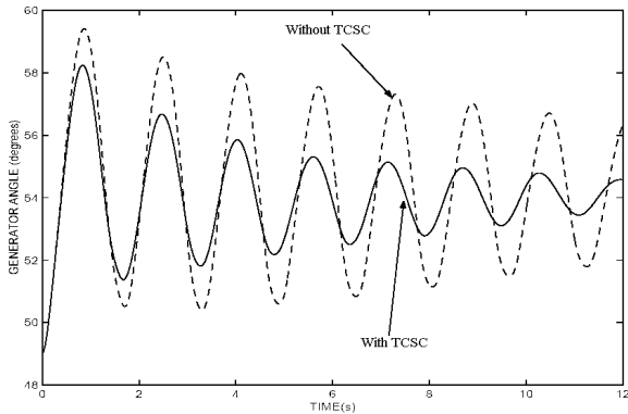
Figure 11: Damping on outage of HVDC line the voltage based controller on MATLAB.
