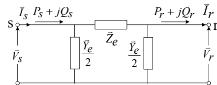
Figure 2: Equivalent \pi circuit model of a transmission line.
