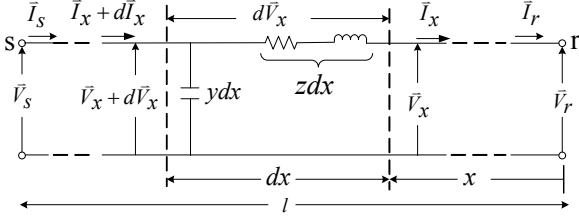
Figure 1: Transmission line model.
