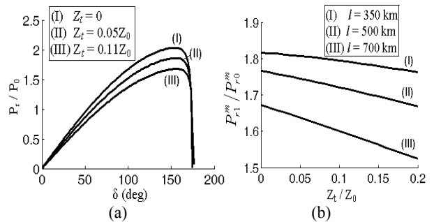
Figure 5: Effect of line terminal impedances on (a) the P_r - \delta characteristic and (b) the steady-state stability limit of a midpoint compensated line.
