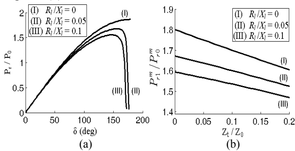
Figure 6: Effect of line resistances on (a) the \delta - P_r characteristic and (b) reducing the benefit under dynamic midpoint compensation
