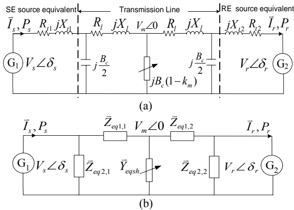
Figure 3: Equivalent circuit of a radial line with midpoint compensation and source impedances.
