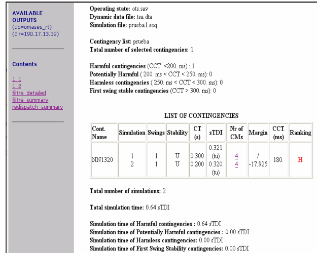
Figure 6: FILTRA output for the modified case
