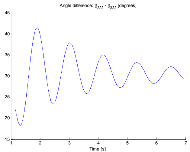
Figure 9: Voltage angle difference between bus 222 and 322
