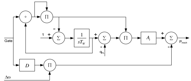
Figure 4: Hydro turbine system model
