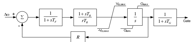
Figure 5: Hydro governor system model
