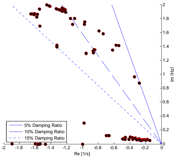
Figure 7: Electro-mechanical modes
