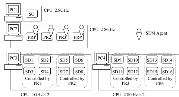
Figure 5: Computer network environment for SDM agent.
