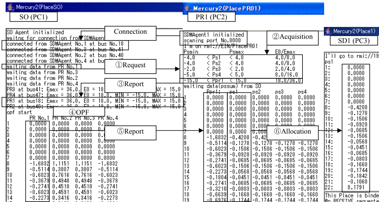
Figure 6: Computer screens of the system operator, Power Router #1 and storage device #1.
