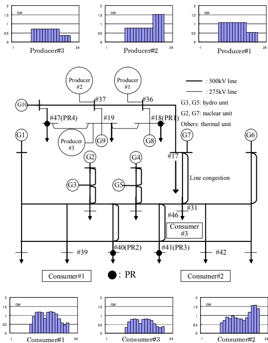
Figure 4: IEEJ East 10-machine system model including bilateral transactions.
