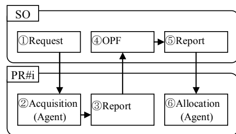
Figure 2: Scheduling process of distributed energy storage devices.
