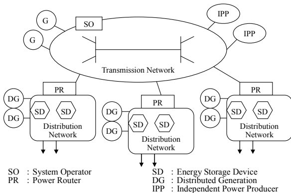
Figure 1: Configuration of a future electric power system.
