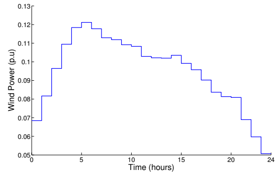
Figure 4: Wind infeed for a day. Wind farm maximum infeed = 0.12 p.u.
