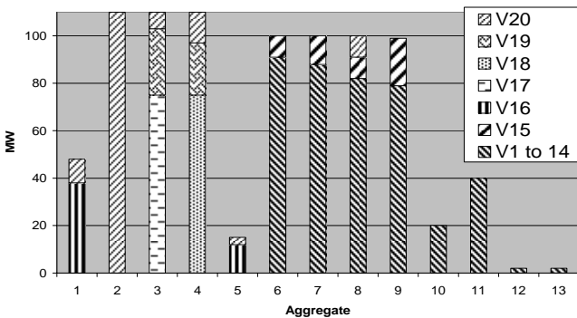
Figure 7: Loading of the units scenario 15 to 20.
