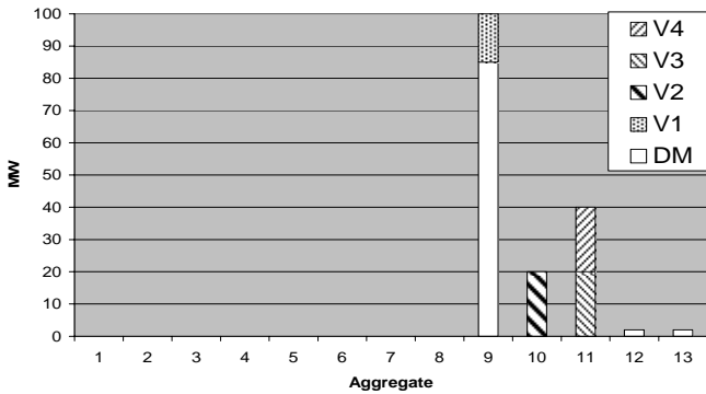
Figure 6: Loading of the units scenario 1 to 4.
