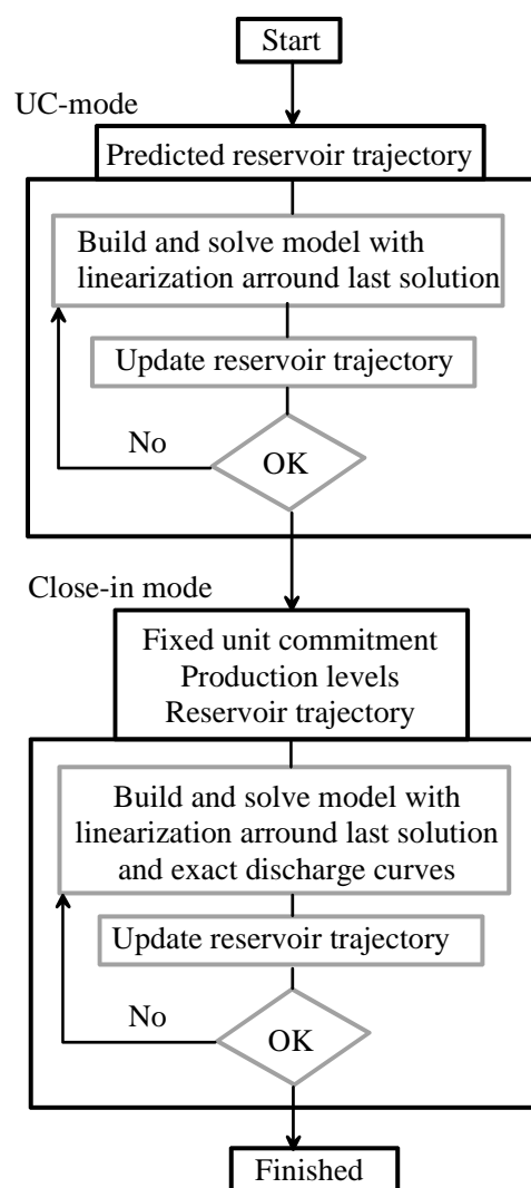
Figure 4: Simplified solution flow diagram for the applied successive linear programming approach.
