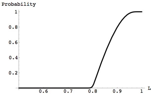
Figure 8: Probability of more than 500 components failed as a function of loading L in CASCADE model. There is a sharp increase at the critical loading L=0.8 .
