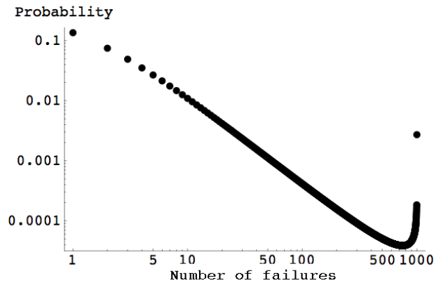
Figure 9: Probability distribution of number of failed components near criticality in CASCADE model.
