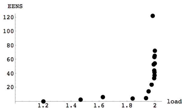
Figure 2: Expected energy not served as a function of the loading factor with respect to the base case. There is a sharp increase in blackout size at the critical loading of 1.94 times the base case loading.
