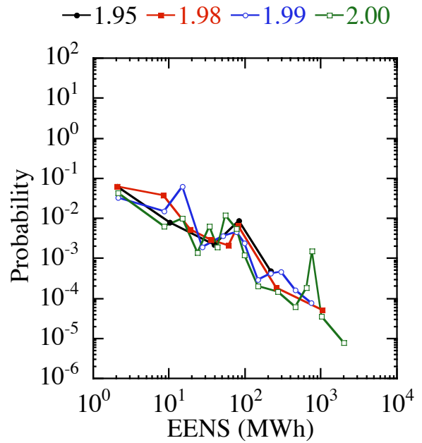
Figure 6: Probability distributions of expected energy not served for four loadings above the critical loading, namely 1.95, 1.98, 1.99 and 2.00 times the base case loading.
