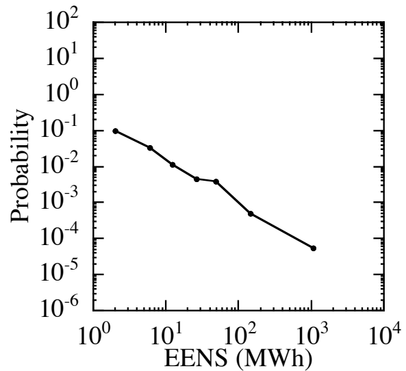
Figure 3: Probability distribution of expected energy not served at the critical loading of 1.94 times the base case loading. Note the log-log scale; a straight line on this plot indicates a power law relation. The straight line slope of approximately -1.2 indicates that the blackout probability is proportional to (\text{EENS})^{-1.2} .
