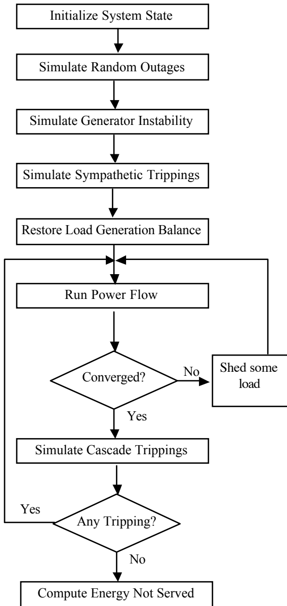
Figure 1: Cascading failure power system model.
