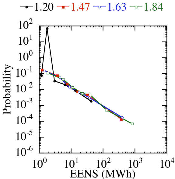
Figure 5: Probability distributions of expected energy not served for four loadings below the critical loading, namely 1.20, 1.47, 1.63 and 1.84 times the base case loading.
