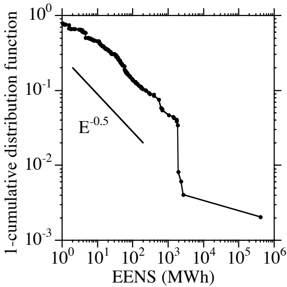
Figure 4: Probability that blackout exceeds a given expected energy not served (complementary cumulative probability distribution) at the critical loading of 1.94 times the base case loading. The straight line slope of approximately -0.5 indicates that the blackout probability is proportional to (\text{EENS})^{-1.5} .
