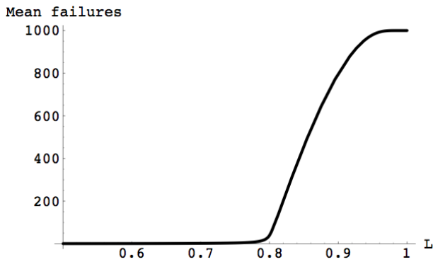
Figure 7: Mean number of failed components as a function of average initial loading L in CASCADE model. There is a sharp increase at the critical loading L=0.8 . There is saturation with all 1000 components failed at loading L=0.96 .
