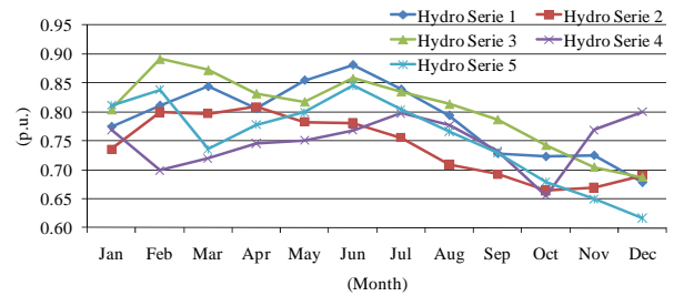
Figure 4: Hydro Monthly Variation.
