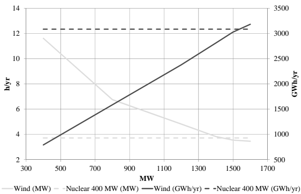
Figure 5: LOLE vs Expected Maximum Energy Produced.
