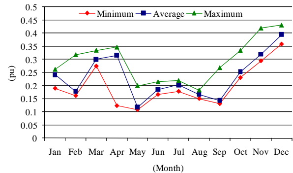
Figure 5: Wind Monthly Variation.
