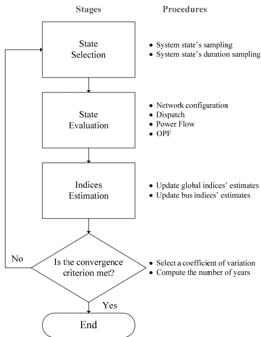
Figure 1: Sequential Monte Carlo Stages and Procedures.
