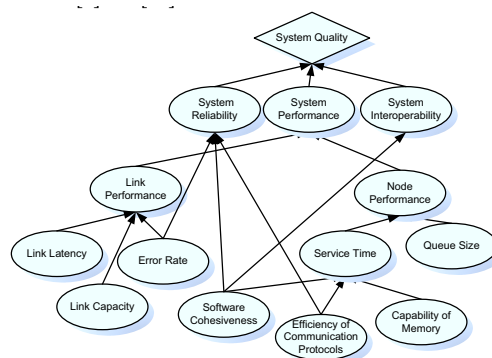
Figure 3: Influence Diagram illustrating the causal relation between attributes that constitute several non-functional aspects of ICT systems[21]
