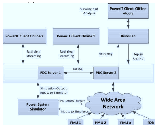
Figure 6: Overview of KTH PowerIT experimental system architecture[26]
