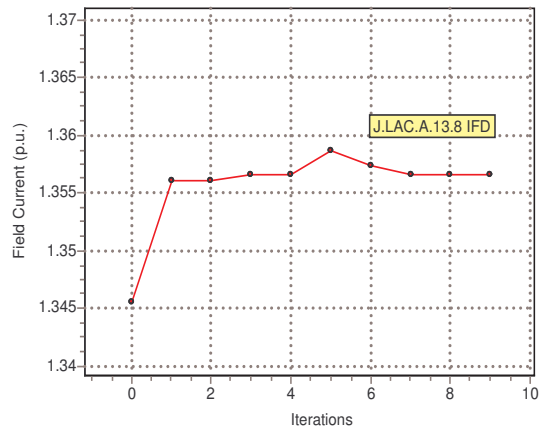
Figure 13: J.Lacerda field current
