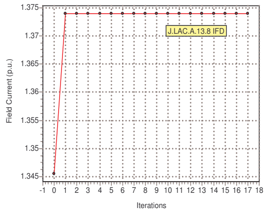
Figure 14: Limits on field current
