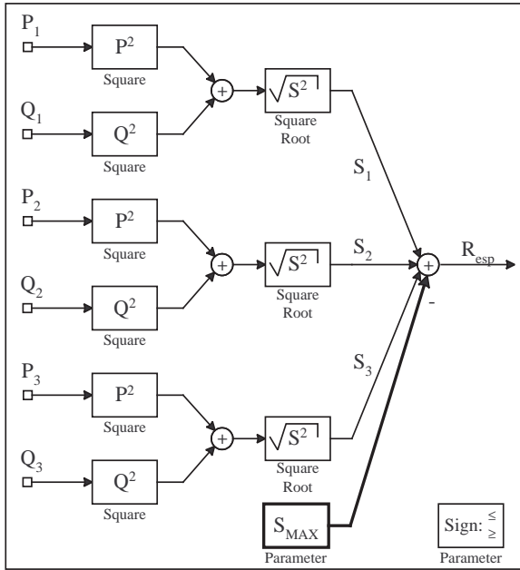
Figure 8: Model of functional constraint
