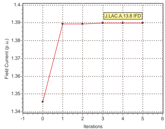
Figure 10: J.Lacerda field current
