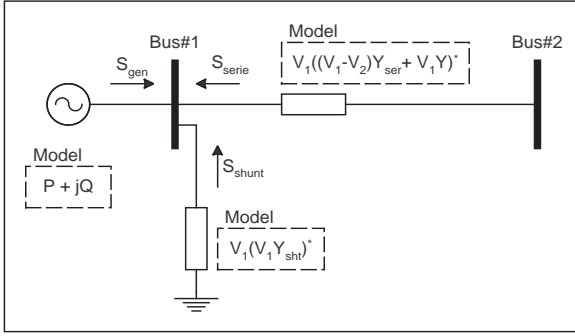
Figure 6: Power balance equations
