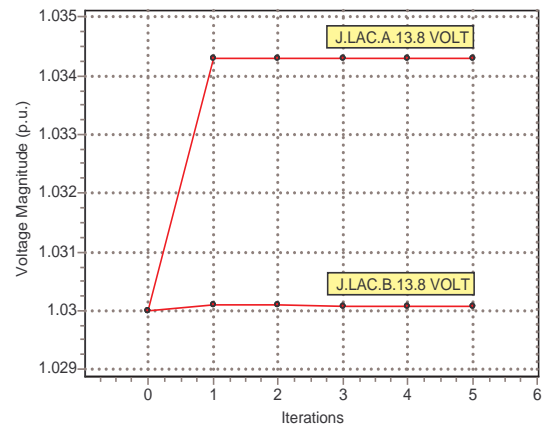
Figure 9: J.Lacerda voltage magnitude
