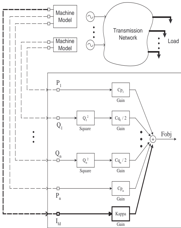
Figure 11: Objective function and synchronous machine models
