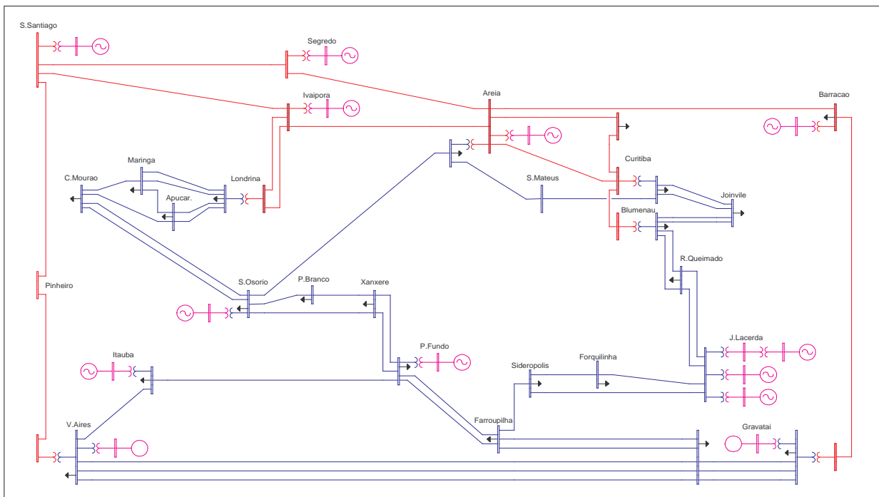
Figure 15: One line diagram of the Brazilian Southern System
