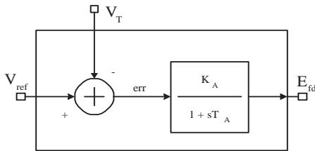
Figure 2: Automatic voltage regulator model
