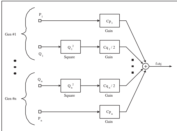
Figure 4: Block diagram representation of the objective function described in equation 3
