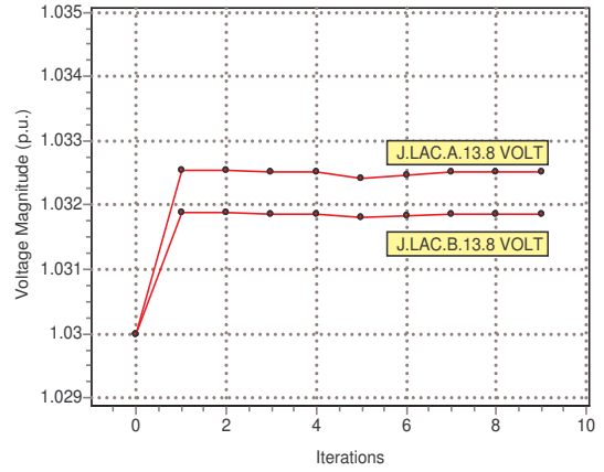
Figure 12: J.Lacerda voltage magnitude
