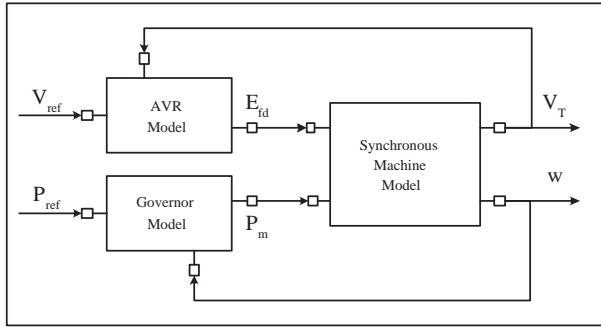
Figure 1: Functional representation of the synchronous machine and its control systems
