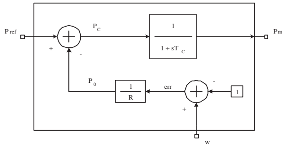
Figure 3: Speed governor model
