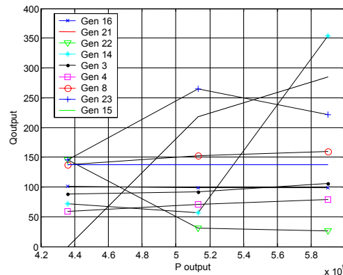
Figure 10: Production expected for each generator
