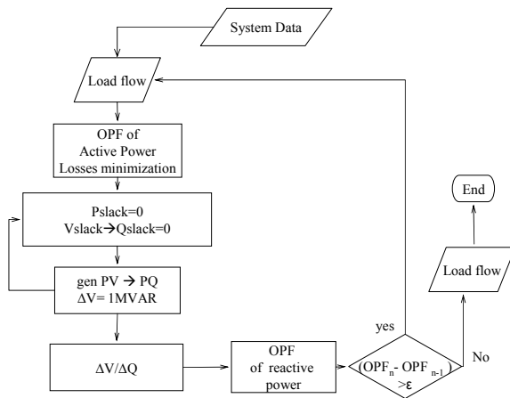
Figure 4: Flow diagram of reactive power optimization
