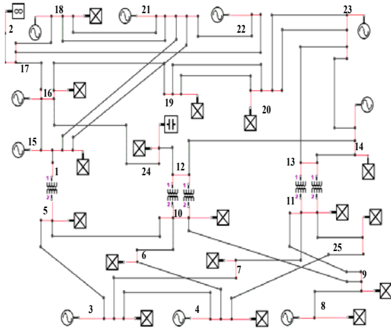
Figure 8: 25 buses Test system (CIGRE modified)
