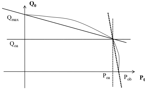
Figure 3: Capability curve for a generator.
