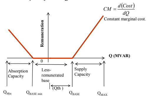
Figure 1: Cost function reactive power production
