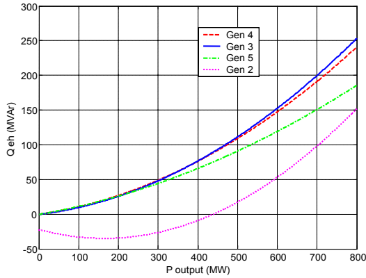
Figure 6: Curve Qth for 13-bus system
