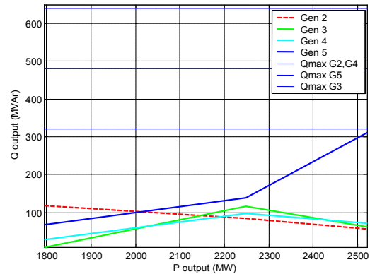
Figure 7: Reactive power production for each generator
