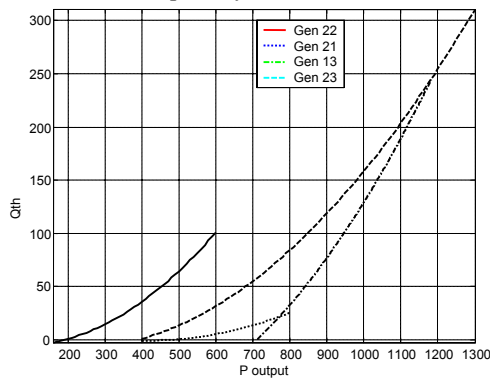
Figure 9: Curve Q_{th} for 24 bus test system CIGRE
