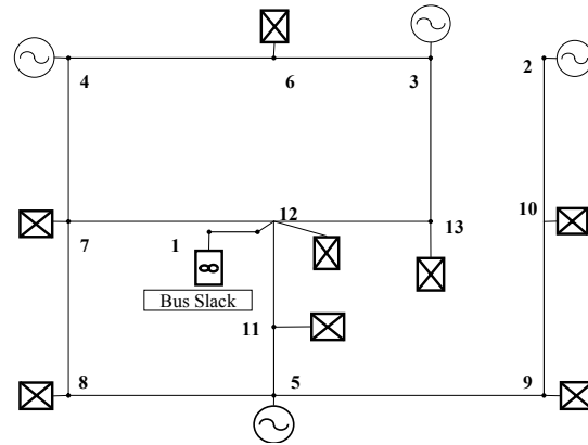
Figure 5: 13-bus system
