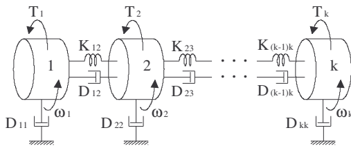
Figure 2: Spring-mass model the turbine shaft coupled to the generator.
