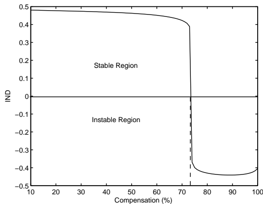
Figure 4: IND values at first iteration.
