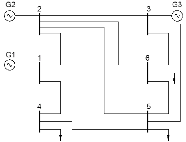
Figure 3: Modified 6-bus test system
