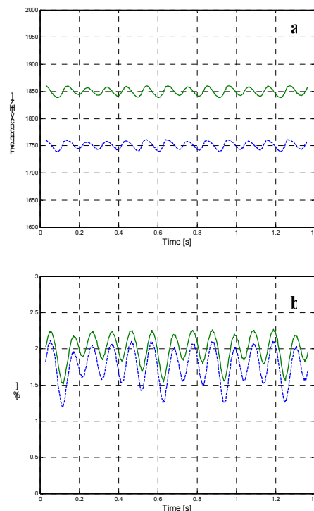
Figure 7: Time-varying frequency (a) and relative amplitude (b) (relative to the mean amplitude over the analysis interval) of MV voltage without compensation at the 1600-2000 Hz band.
