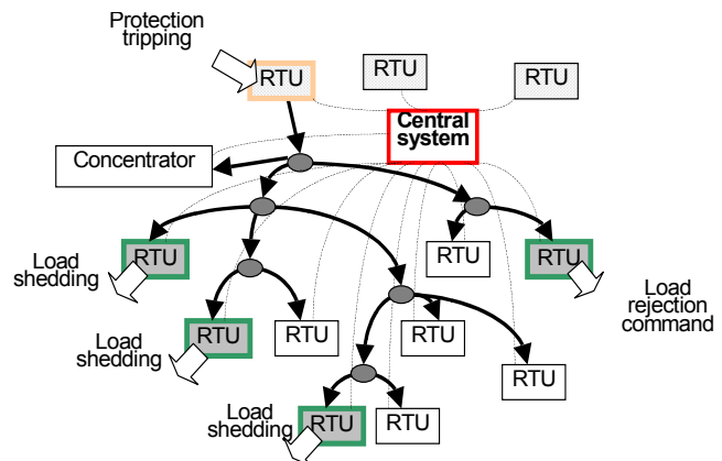
Fig. 2: Flow of actions following the detection of an occurred critical event.
