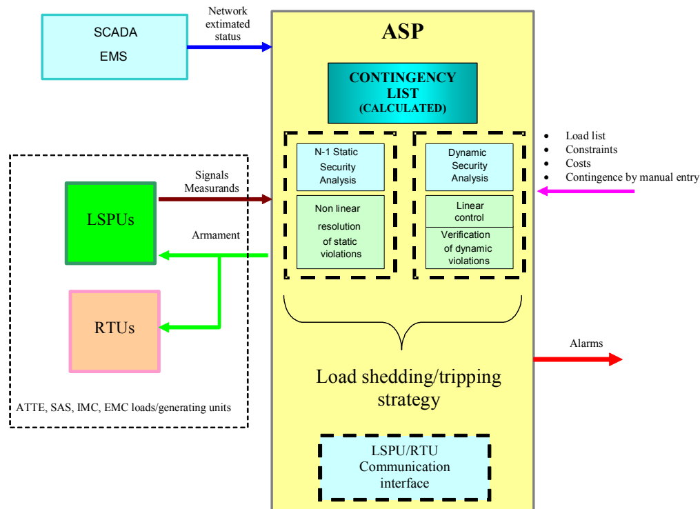
Fig. 1 – Overall architecture of the Automatic Shedding Processor (ASP): on the left side it is shown the interconnection of existing ATTE, SAS, EMC and IMC (exchanging with Load Shedding Peripheral Units - LSPU - and Remote Terminal Units RTU: tele-measurements TM, tele-signals TS, alarms and rules), on the right side it is shown the architecture of SSA and DSA modules, providing ESAS-Analysis and ESAS-Control functions, acquiring information from SCADA and EMS (state estimation), and exchanging data with ATTE, SAS, EMC and IMC (load configuration and measurements, control rules and sensitivity data).
