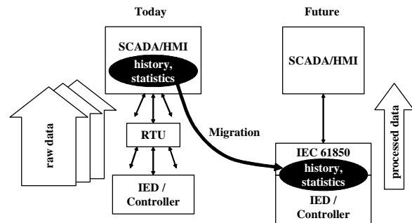
Figure 2: Migration of processing to IEDs
