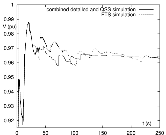
Figure 7: Simulation of marginally stable case
